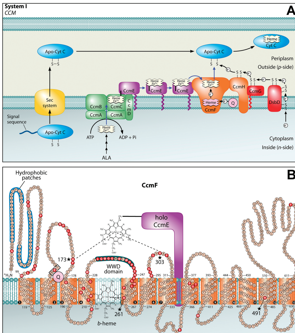
Figure 1. (A) Current working model of the system I cytochrome c biogenesis pathway. Model includes trafficking and oxidation states of heme as well as the subpathways for apocytochrome translocation and reduction. (B) Topology of the CcmF integral membrane protein from E. coli . Possible histidine axial ligands to heme are starred. The highly conserved WWD domain is shaded as are the hydrophobic patches. Completely conserved amino acids (red) were identified by individual protein alignments using CcmF ORFs from the following organisms: the alpha proteobacteria, Agrobacterium tumefaciens CS8, Rhodobacter capsulatus , Caulobacter crescentus CB15, and Bradyrhizobium japonicum ; the beta proteobacteria, Nitrospira multiformis ATCC 25196 and Nitrosomonas europaea ATCC 19718; the gamma proteobacteria, Escherichia coli K-12 MG1655, Pseudomonas fluorescens Pf01, Shewanella oneidensis MR-1, and Vibrio parahaemolyticus RIMD 2210633; the delta proteobacteria, Myxococcus xanthus and Desulfovibrio desulfuricans ; and the deinococci, Deinococcus geothermalis and Thermus thermophilus . Adapted from ref 5.
