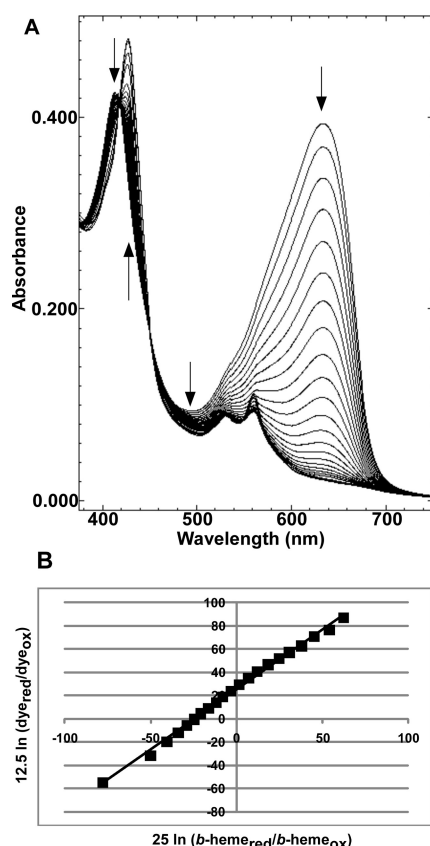
Figure 8. Redox titration of the CcmF b -heme. Spectra collected during a typical reductive titration of CcmF b -heme with nile blue chloride (A) and the corresponding linear Nernst plot (B). Arrows in (A) indicate the direction of changes in absorption during the course of the titration. In (B), [25 \text{ mV} \ln (b\text{-heme}_{\text{red}}/b\text{-heme}_{\text{ox}})] was used for the one-electron reduction of heme and [12.5 \text{ mV} \ln (\text{dye}_{\text{red}}/\text{dye}_{\text{ox}})] was used for the two-electron reduction of dye, where b\text{-heme}_{\text{red}}/b\text{-heme}_{\text{ox}} and \text{dye}_{\text{red}}/\text{dye}_{\text{ox}} represent ratios of the molar concentrations of the reduced and oxidized forms of the b -heme and the dye, respectively. Conditions: 20 mM Tris-HCl, pH 7, 100 mM NaCl, 0.02% DDM.
