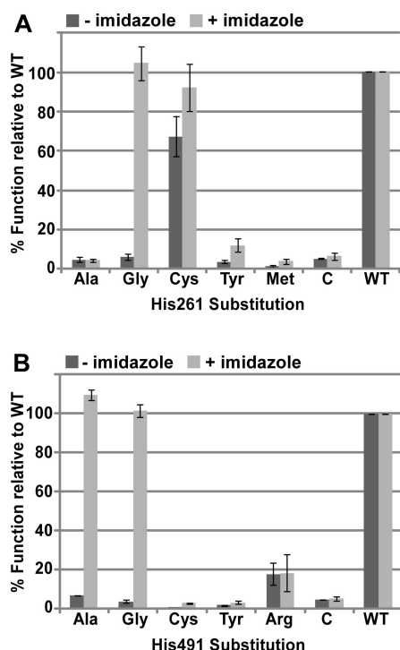
Figure 6. In vivo heme attachment to cytochrome c_4 (i.e., holocytochrome c formation) by the indicated CcmF His261 and His491 mutants in the presence or absence of 10 mM imidazole. The function of each of the indicated substitutions at CcmF His261 (A) or His491 (B) is reported as a percentage of wild-type CcmF (WT) function. Holocytochrome c_4 was quantified by measuring the chemiluminescent heme stain signal of 100 \mu g of BPER-isolated proteins from three independent experiments. Representative heme stains are provided in Supporting Information (Figure S3). Error bars denote standard deviation. "C" denotes control, which represents chemiluminescent signal in the absence of CcmF (any signal lower than the control is considered background).
