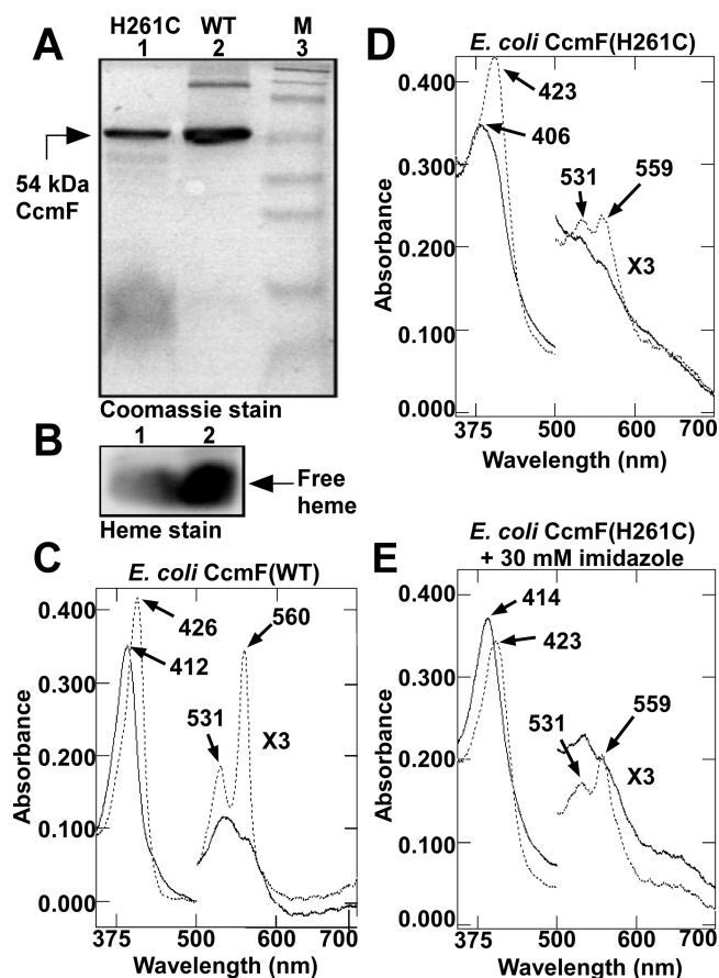
Figure 5. Spectral analysis of CcmF His261Cys (H261C) and wild-type CcmF (WT) proteins. Coomassie stain (A) and heme stain (B) of CcmF(WT) and CcmF(H261C) proteins. UV/vis absorption spectra of CcmF(WT) (C), CcmF(H261C) (D), and CcmF(H261C) in the presence of 30 mM imidazole (E), oxidized (solid lines) and dithionite-reduced (dotted lines). Absorption maxima are indicated with arrows. Absorbance values between 500 and 700 nm have been multiplied by a factor of 3. 30 \mu g of purified protein was analyzed by Coomassie and heme stain (A, B). For UV/vis absorption spectra \sim 20 \mu M purified protein was analyzed for wild-type, and \sim 40 \mu M purified protein was analyzed for His261Cys in the presence and absence of 30 mM imidazole.
