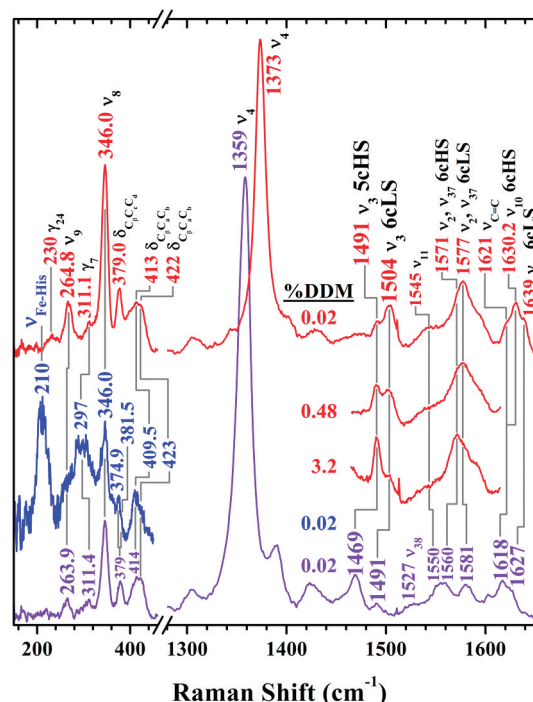
Figure 2. Soret-excited resonance Raman spectra of the heme b in ferric (red) and ferrous (violet, blue) CcmF. Sample solutions were 88 \mu M in holoCcmF, 20 mM in Tris, pH 8, 100 mM in NaCl, 0.02% in dodecyl maltoside, \sim 2 mM in imidazole. HoloCcmF concentrations in the 3.2% and 0.48% dodecyl maltoside samples were 23 and 25 \mu M, respectively. The red and violet spectra were recorded using 10 mW of laser light at 413.1 nm (line focus of emission from Kr + laser). The low-frequency blue spectrum was recorded with 2 mW of 441.6 nm emission from a HeCd laser to identify the Fe–His stretching band.
