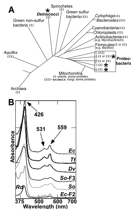
Figure 7. Phylogenetic distribution and spectral analysis of diverse CcmF proteins. (A) Representative distribution of systems I, II, and III among the bacteria and archaea. The system number is noted in parentheses after each group name, and stars indicate groups containing organisms from which recombinant hexahistidine-tagged CcmF was analyzed in the present study. Adapted from ref 23. (B) Reduced UV/vis absorption spectra of CcmF from E. coli (Ec), Thermus thermophilus (Tt; Deinococcus group), Desulfovibrio vulgaris (Dv), Roseobacter denitrificans (Rd), and Shewanella oneidensis (So); Shewanella oneidensis CcmF-3 (So-F3), and E. coli CcmF-2 (Ec-F2). Absorption maxima are indicated with arrows. Spectra have been offset for clarity. Approximately 20 \mu M of each purified CcmF protein was analyzed for which Coomassie and heme stains are provided in Supporting Information (Figure S4).
