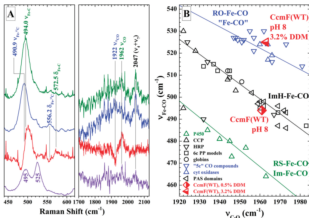
Figure 3. (A) Soret (413.1 nm)-excited rR spectra of natural abundance CcmF-CO (green) and CcmF- 13 CO (blue) in the \nu_{\text{Fe-C}} and \nu_{\text{C-O}} frequency regions. The red traces are the difference spectra, whose amplitudes have been multiplied by a factor of 2 for ease of viewing. The difference features reveal the bands whose frequencies are 13 C dependent, thereby facilitating their assignments to FeCO modes, which are indicated in the labels above the bands. The violet trace shows the spectrum of natural abundance CcmF-CO in 3.2% DDM. Note that this spectrum exhibits two Fe-C stretching bands. This heterogeneity is attributed to protein conformational changes driven by the high detergent concentration. (B) Heme FeCO backbonding correlation plot showing the positions of the two CcmF-CO conformers. The CcmF-CO complex that falls on the middle line (0.48% DDM) most likely contains a proximal imidazole ligand from a His residue. Its position low and to the right on the imidazole line shows that the CO ligand interacts only weakly with the heme pocket. The CcmF-CO complex that falls on the top line (3.2% DDM) is either pentacoordinate or has a proximal ligand that is bound through an oxygen atom.
