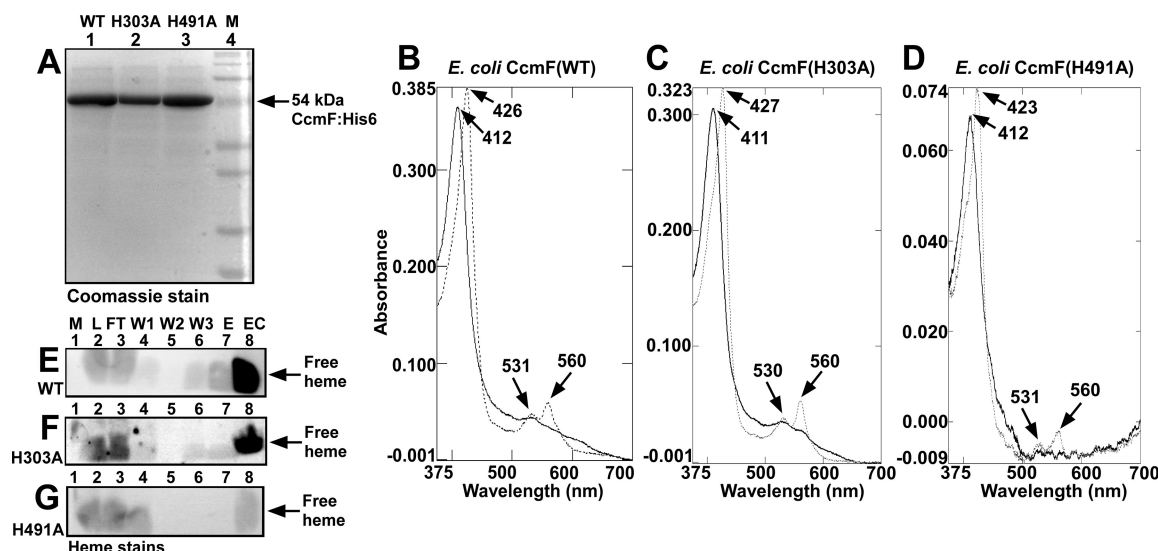
Figure 4. Heme levels in E. coli wild-type CcmF (WT), CcmF His303Ala (H303A), and CcmF His491Ala (H491A) proteins. Coomassie stain (A) of CcmF(WT), CcmF(H303A), and CcmF(H491A) showing purified full-length 54 kDa proteins (indicated by arrow). UV/vis absorption spectra of CcmF(WT) (B), CcmF(H303A) (C), and CcmF(H491A) (D) as purified (oxidized; solid lines) and dithionite-reduced (dotted lines). Absorption maxima are indicated with arrows. Heme stains of CcmF(WT) (E), CcmF(H303A) (F), and CcmF(H491A) (G); free heme is indicated with arrows; M, molecular weight standards; L, load; FT, flow-through; W1–W3, washes 1–3; E, elution; EC, concentrated elution, as described in Experimental Procedures. 20 \mu M purified CcmF protein was analyzed by UV/vis absorption spectroscopy (B, C, D), and 30 \mu g was analyzed by heme stain or Coomassie stain (A; E, F, G, lane 8).
